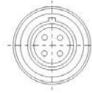
Cable connector Mate with DELMSF811, DELMSF812
