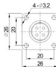
Square flange Mate with DELMSF1610
