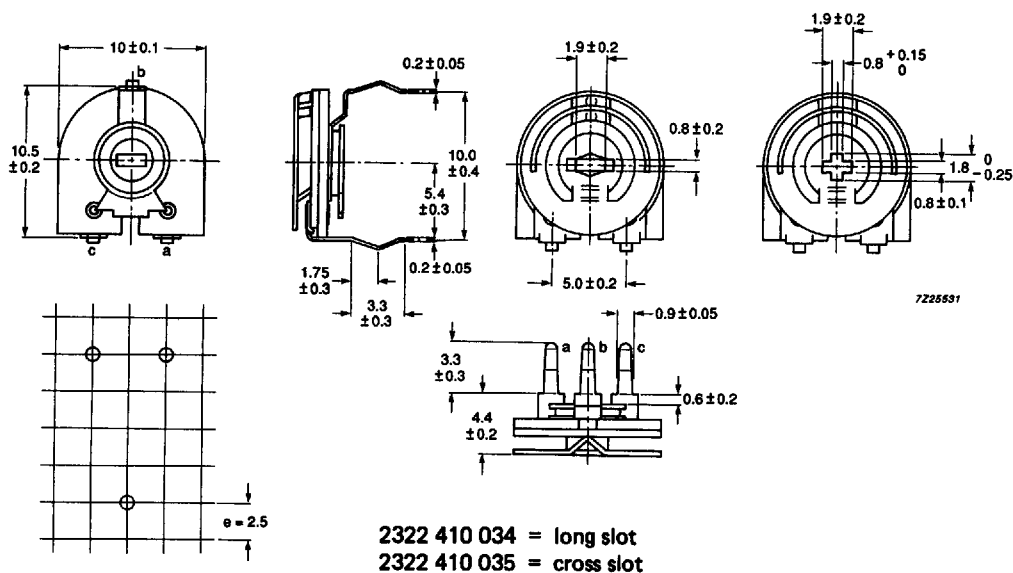
Fig.8 Potentiometers for horizontal mounting: snap-in pins.
