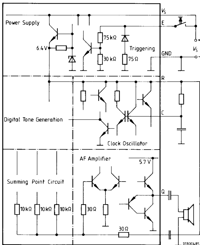
Figure 1 Block Diagram
