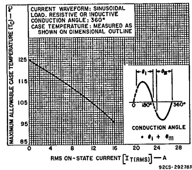
Fig. 2 — Maximum allowable case-temperature vs. on-state current.
